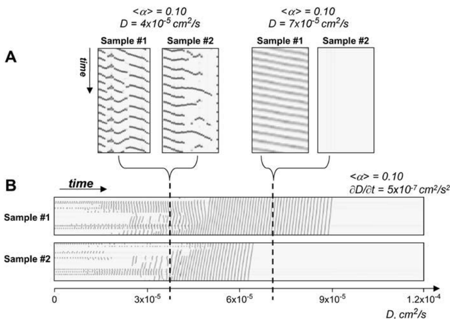
FIGURE 15 Difference in spatial distribution of \langle\alpha\rangle and its effect on network behavior and transitions between the states. (A) x, t scans acquired for two spatially different distributions of \langle\alpha\rangle (each with \delta\alpha/\langle\alpha\rangle = 1/2 ) for two sets of conditions \langle\alpha\rangle = 0.1 ; D = 4 \times 10^{-5} and \langle\alpha\rangle = 0.1 ; D = 7 \times 10^{-5} . (B) x, t scans acquired during the transition from D = 0 to D = 1.2 \times 10^{-4} at fixed \langle\alpha\rangle = 0.10 . Each transition scan corresponds to a different spatial distribution of \alpha(i, j) . Dotted lines point to the relative positions of the x, t scans shown in A within the scope of the entire transition.
