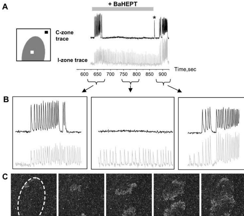
FIGURE 3 Effect of \text{BaCl}_2 -Heptanol application to the I -zone. (A) Diagram on the left depicts position of the I - and C -zones, and regions of interest used to acquire traces on the right. The shaded trace illustrates continuous activity within I -zone during the entire period of \text{BaCl}_2 -Heptanol application and its wash-out. In contrast, the only two periods when activity was present in the C -zone are the wash-in and wash-out of the \text{BaHept} . During \text{BaCl}_2 -Heptanol application itself, no activity is recorded in the C -zone with the exception of the occasional single beats (marked by an asterisk), associated with intrinsic low-frequency spontaneous activity of the layer. (B) Extended traces from the figure above. Periods associated with wash-in, continuous application and wash-out of \text{BaCl}_2 -Heptanol are shown. (C) Appearance of the events in x,y mode during \text{BaCl}_2 -Heptanol application. The dotted oval shows the position of the I -zone. This sample sequence of five frames shows two colliding ectopic waves. The changing pattern of propagating ectopic waves remained confined to the I -zone until wash-out of \text{BaCl}_2 -Heptanol application was initiated.
